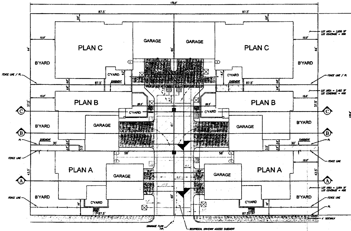
6-PAK CLUSTER PLAN SCALE: 1"=10'
