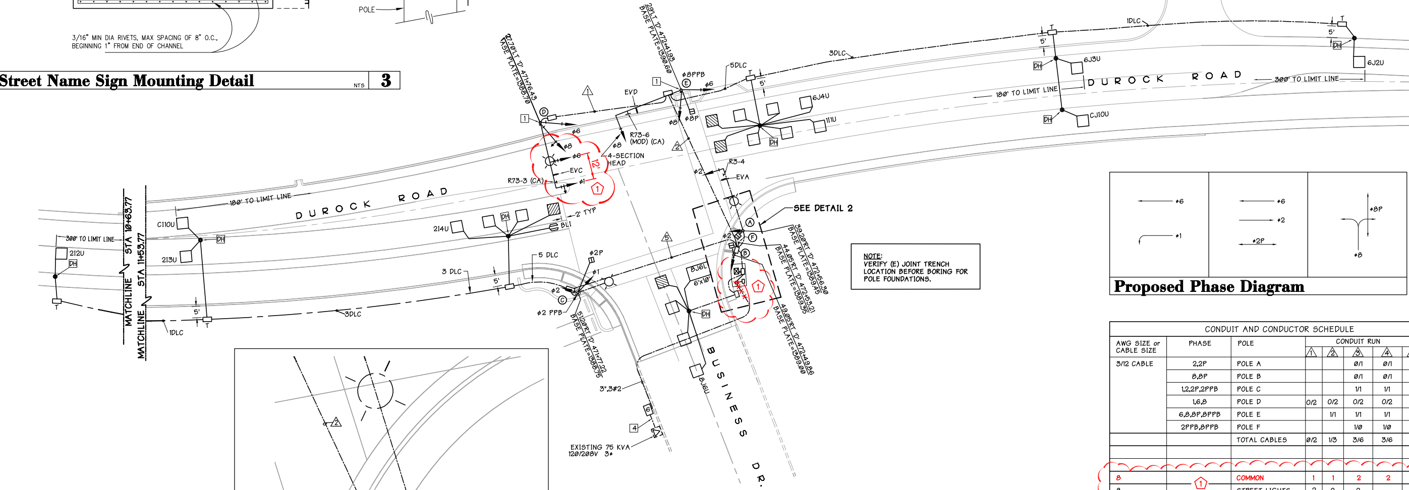
Plan View 1"=20'
