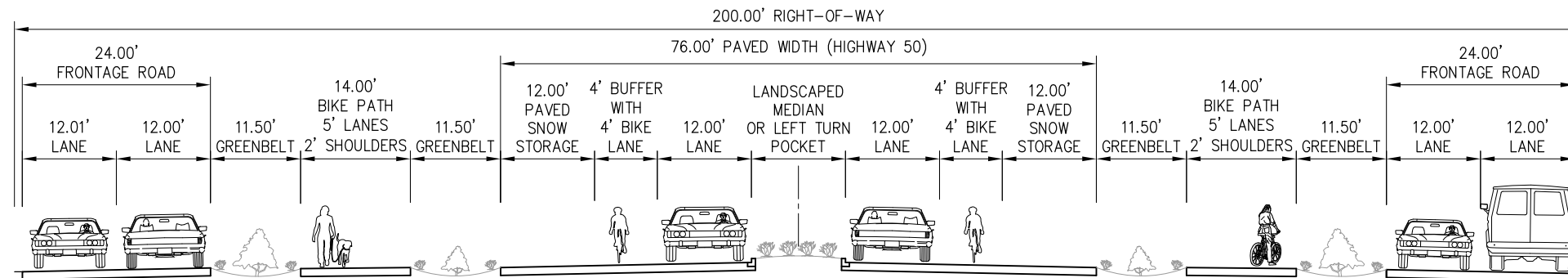
CONCEPT 2: TWO-WAY FRONTAGE ROADS
