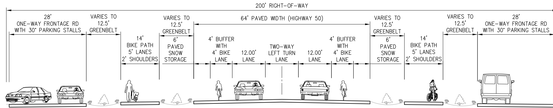
CONCEPT 1: ONE-WAY FRONTAGE ROADS
