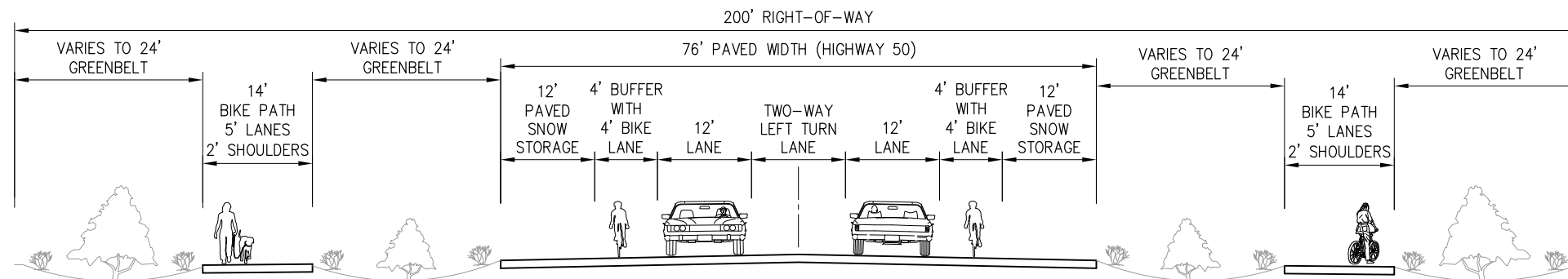
CONCEPT 3: NO FRONTAGE ROADS
