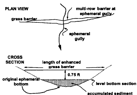
Figure 1. Two row barriers in concentrated flow areas must extend long enough to avoid bypass around the ends at high flow.
